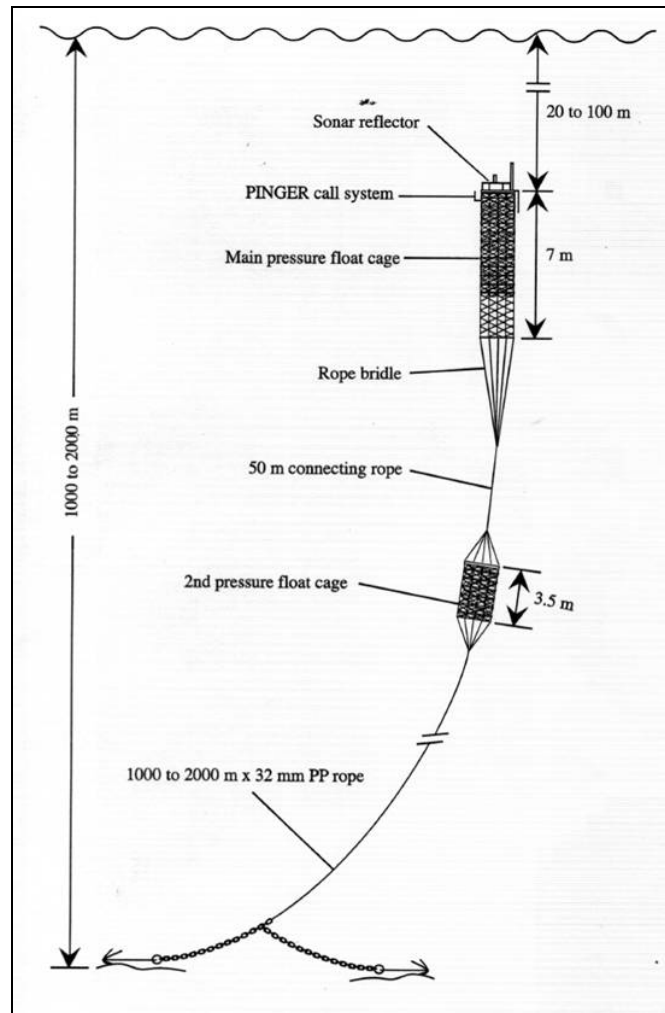
Figure 24. Midwater FAD.
