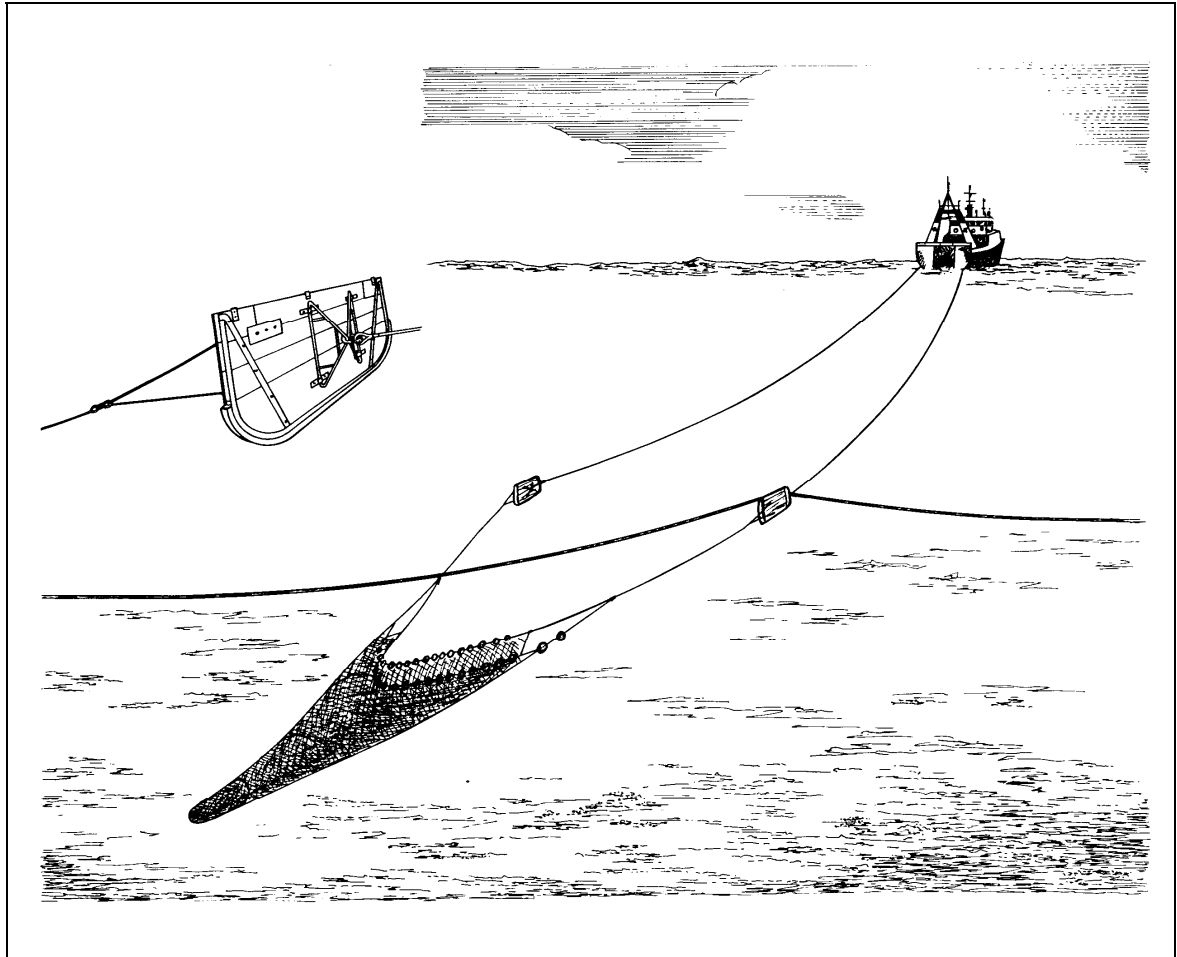
Figure 12. Bottom (otter) trawl catching cable
