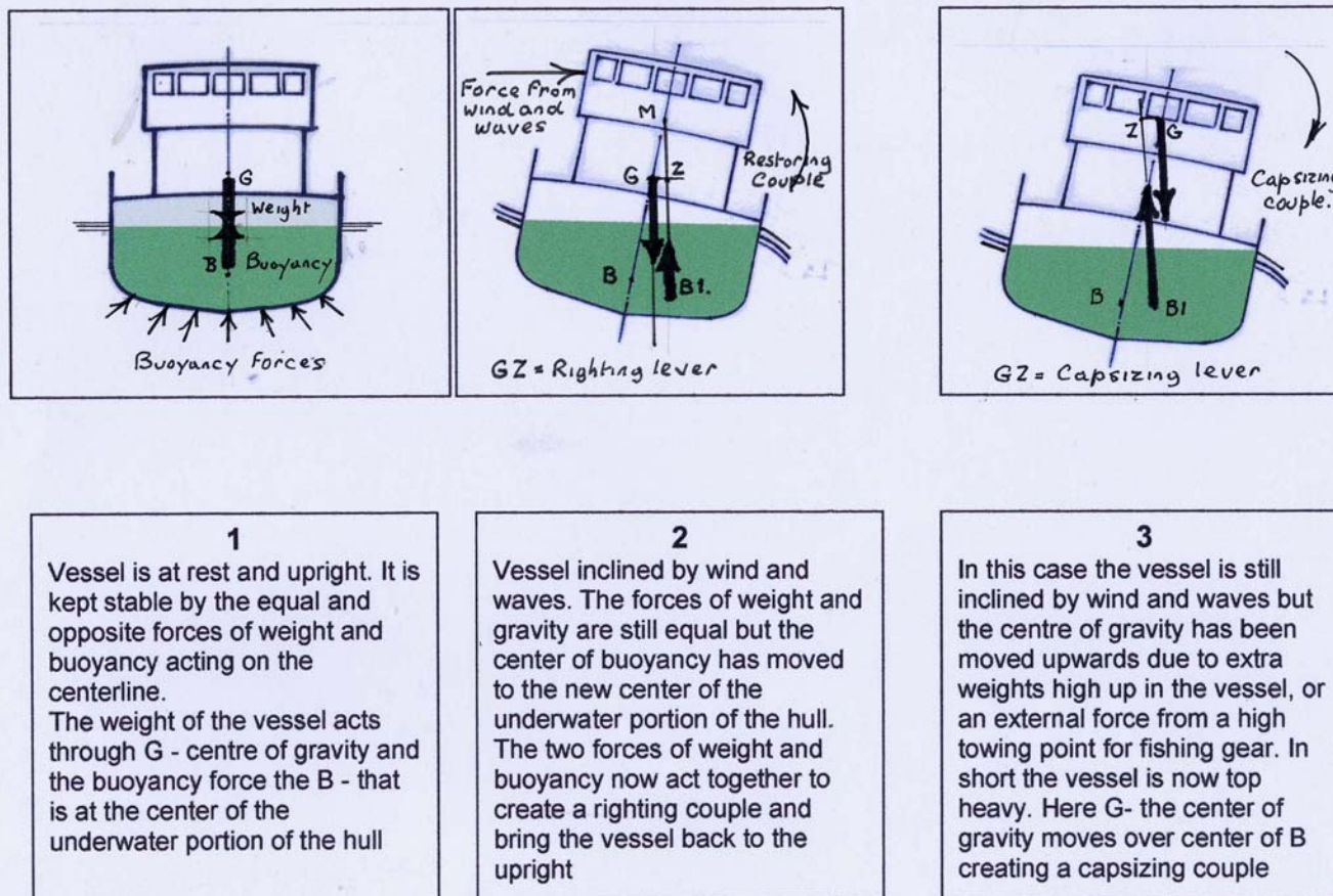
Figure 25. Basics of Stability of Fishing Vessels
