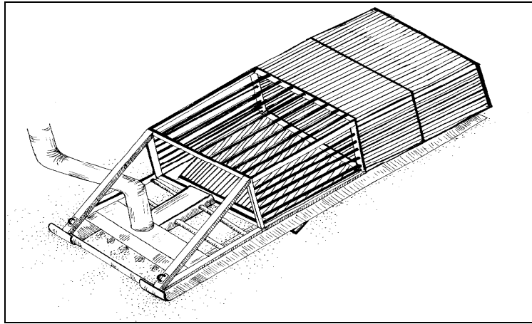
Figure 19. Mechanised (hydraulic) clam dredge.
