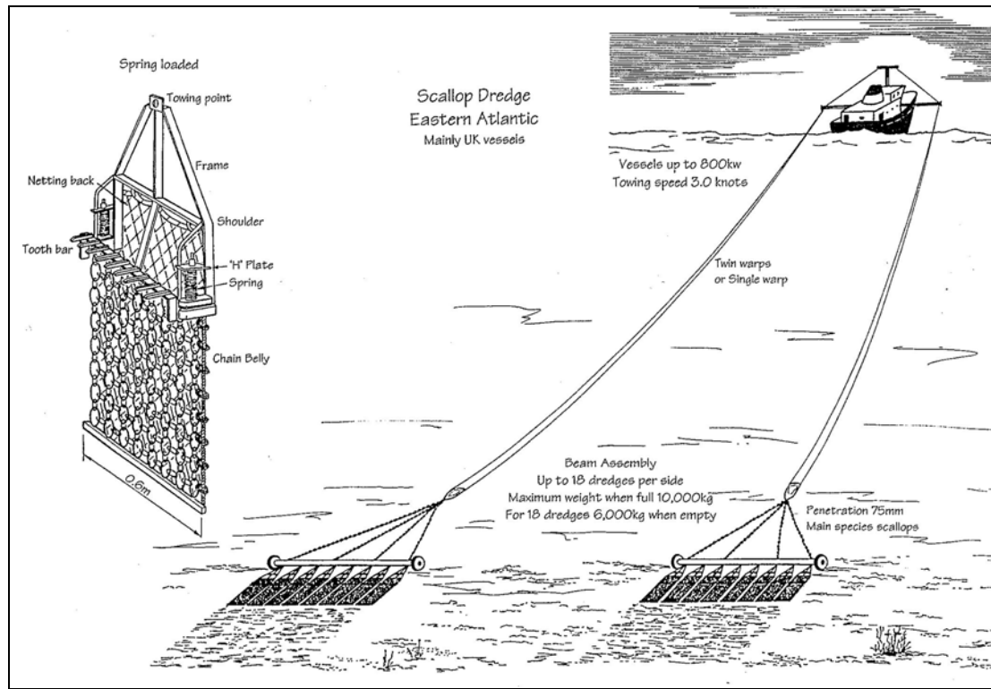
Figure 18. Scallop dredge, European type.
