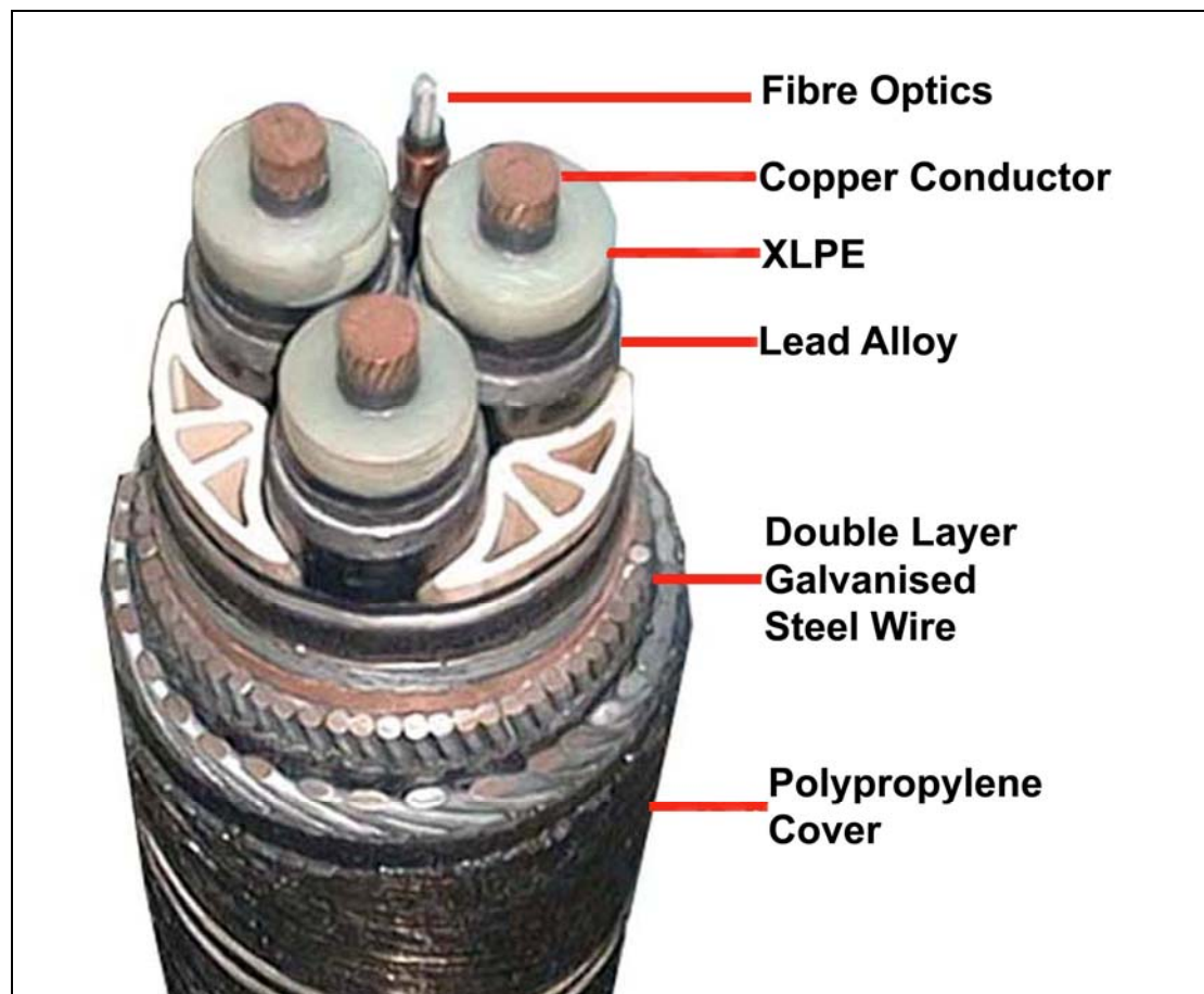
Figure 4. High Voltage (HV) AC Cable, 300 mm (12 inch) diameter
