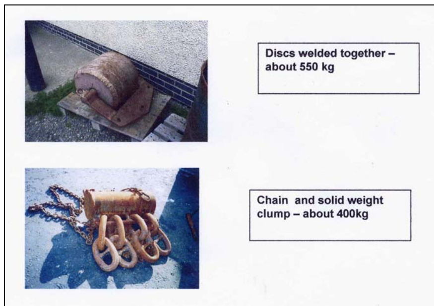
Figure 14. Examples of clumps used in twin/triple trawls
