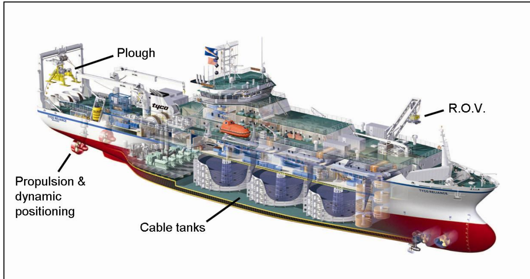
Figure 6. Cables ship Cutaway
