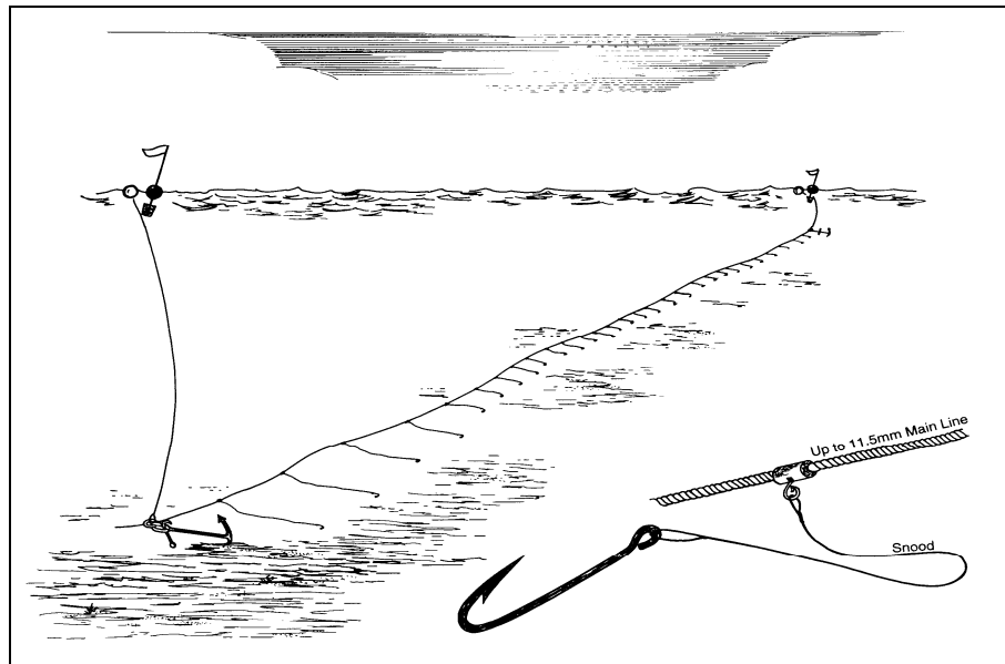
Figure 20. Bottom longline.
