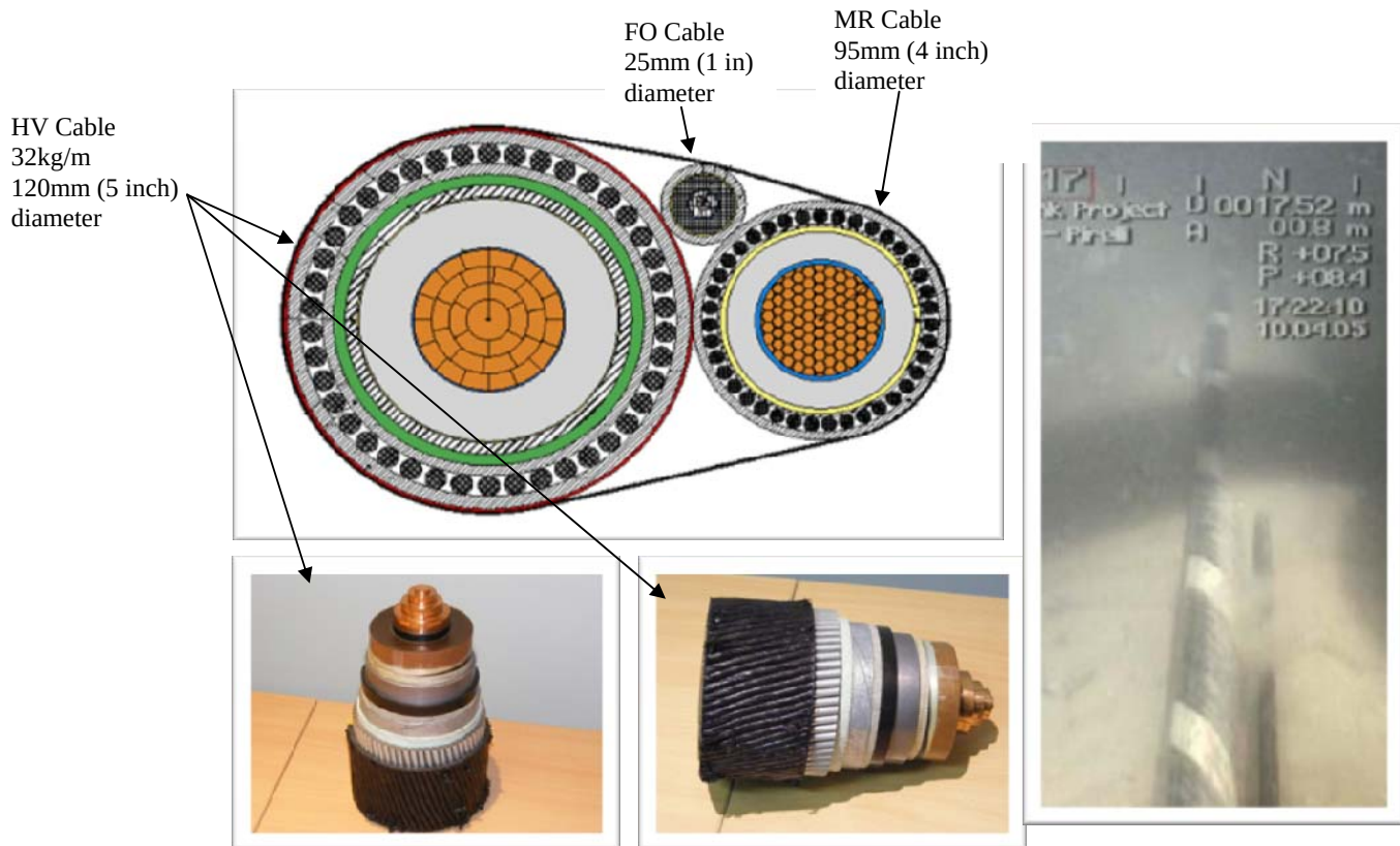
Figure 5. High Voltage DC Cable
