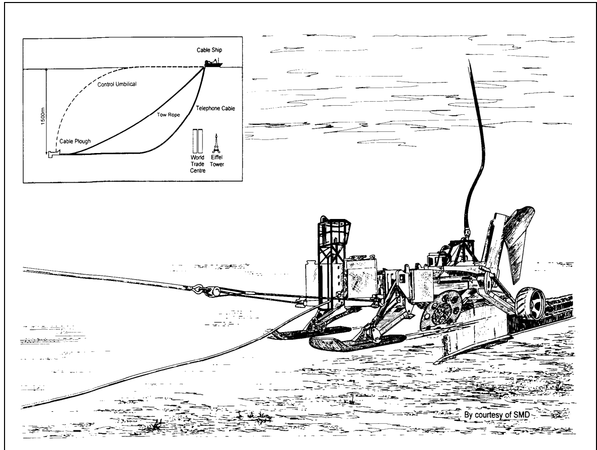
Figure 8. Plough for cable burial, courtesy SMD
