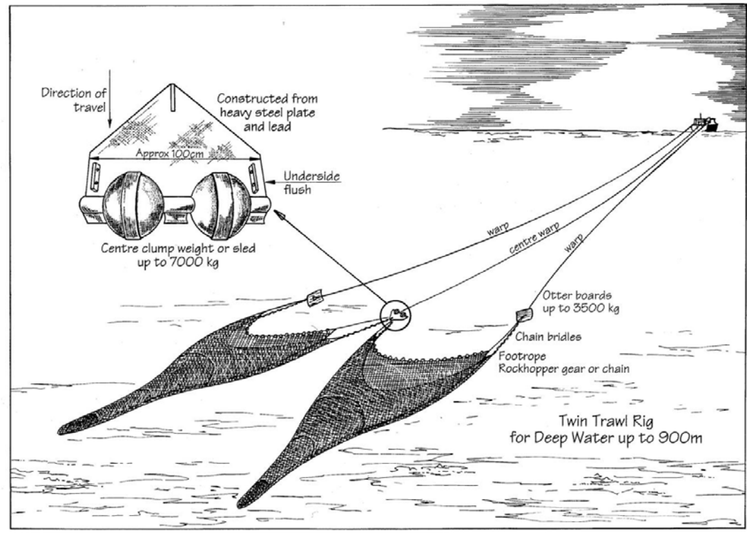
Figure 13. Twin trawl rig.
