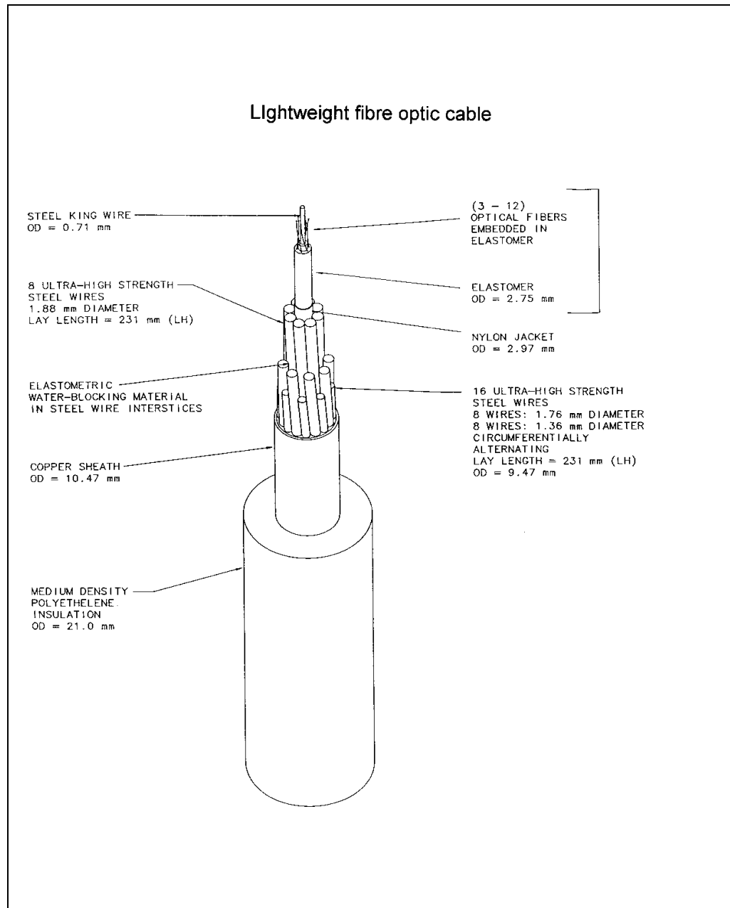
Figure 2. Lightweight Fibre Optic Cable
