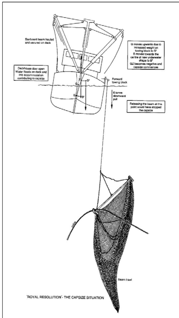
Figure 28. Capsize situation
