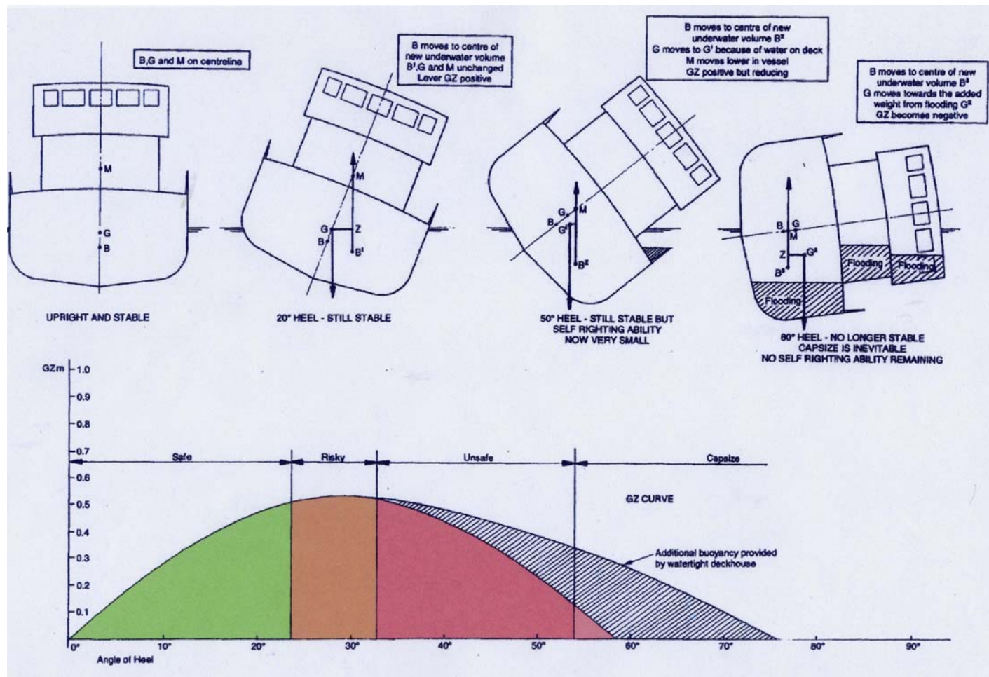
Figure 26. The physics of capsize
