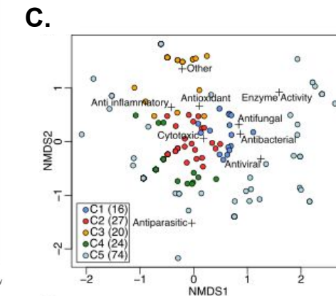
Figure 2. A. A phylogenetic map of bioactivity in the deep sea. B. Using a skelspheres descriptor with a 90% similarity index, links and positioning show structural similarity of structural scaffolds of novel and bioactive chemistry sourced from the deep sea. C. An NMDS plot of taxonomy, environment and bioactivity clusters.
